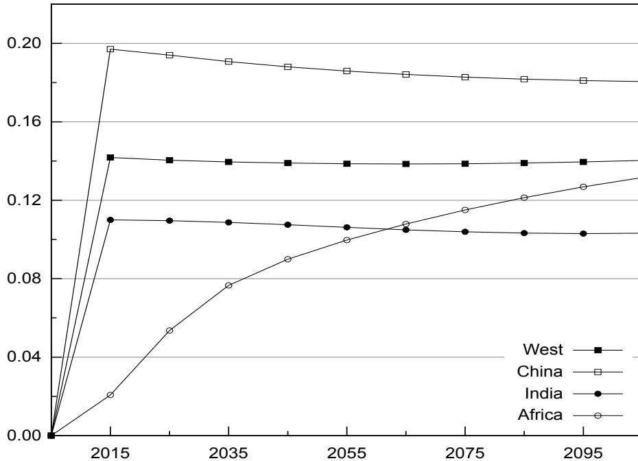
Figure 9: Relative deviation of \mu^c from benchmark when \chi^{ac} is increased by 50%, 2005–2105
